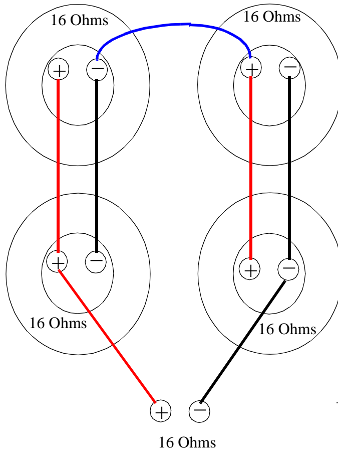
Series-Parallel Wiring
