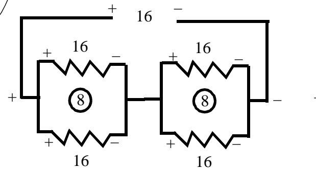
Schematic View
